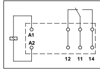
Pin assignment: view of the connections.
